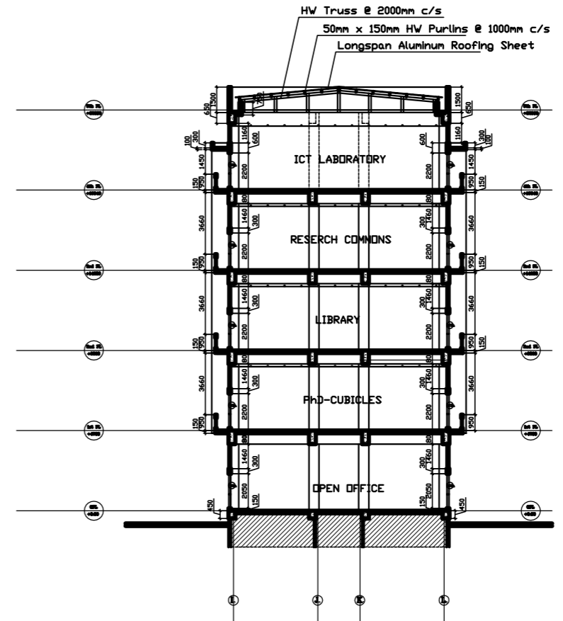
SECTION C.-C.
